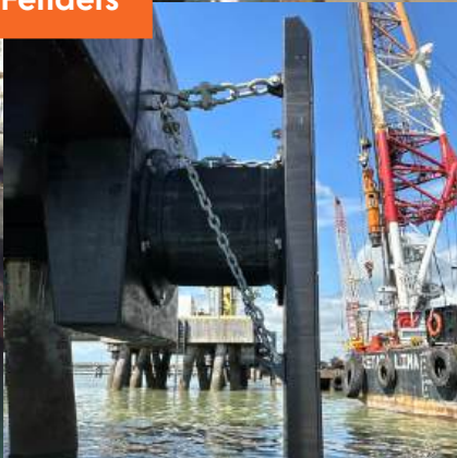
Marine Fenders
